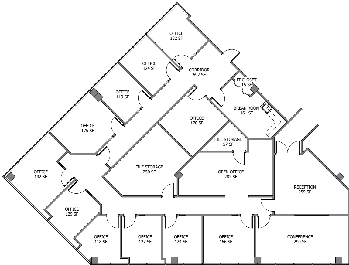
FLOOR PLATE
